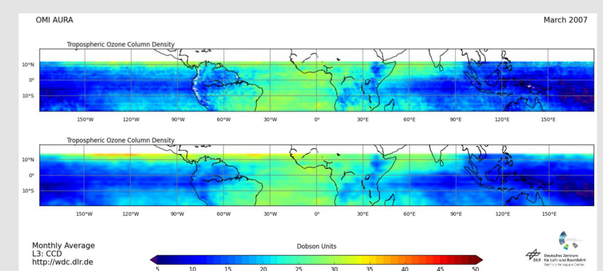
Fig 6: Tropospheric ozone columns from OMI for March 2007 with a fine resolution (top) and low resolution (bottom)
