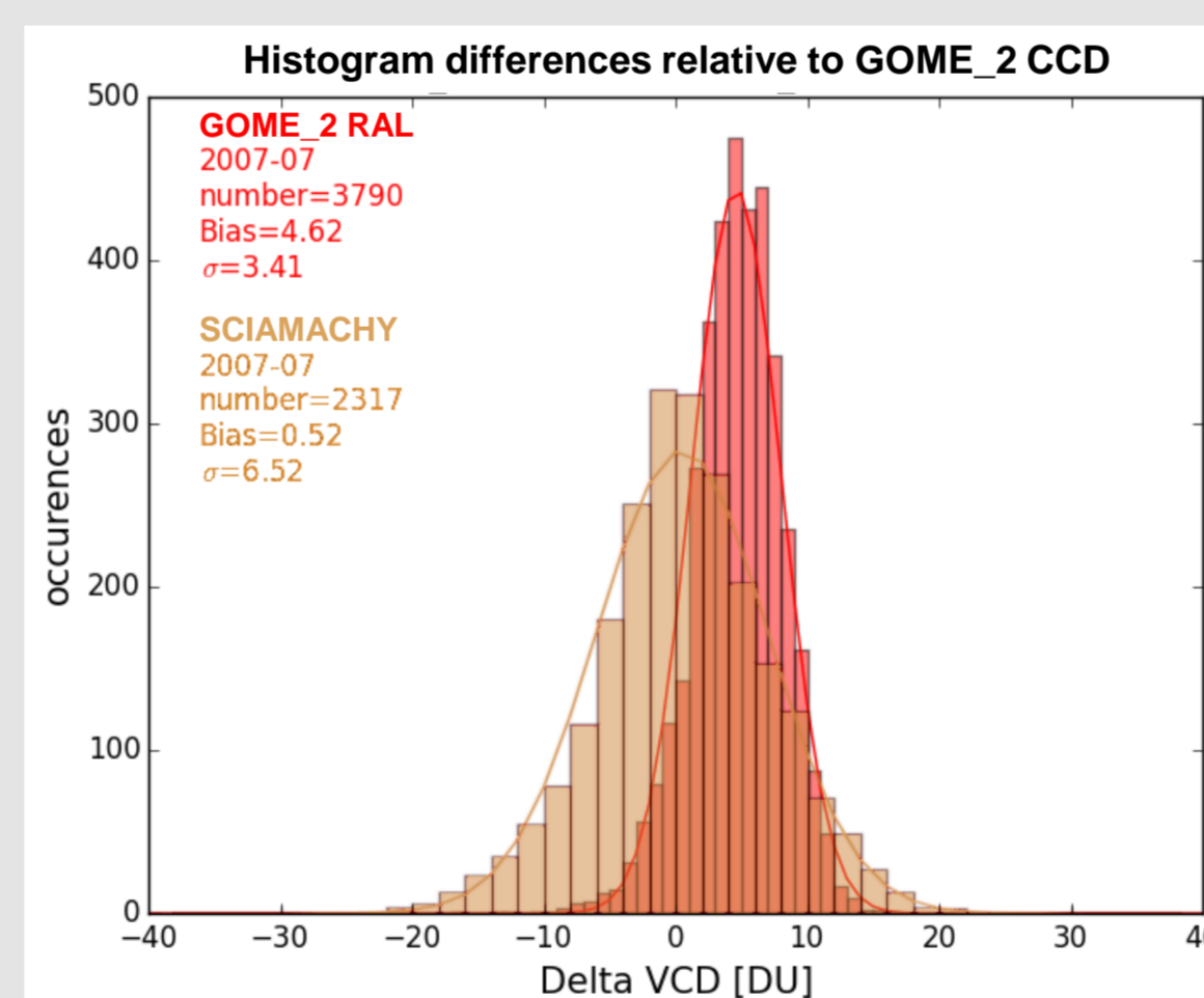
Fig 4: Histogram of the differences between GOME_2 CCD and GOME_2 RAL or SCIAMACHY. For July 2007 the standard deviations are 3.4 and 6.5 DU.
