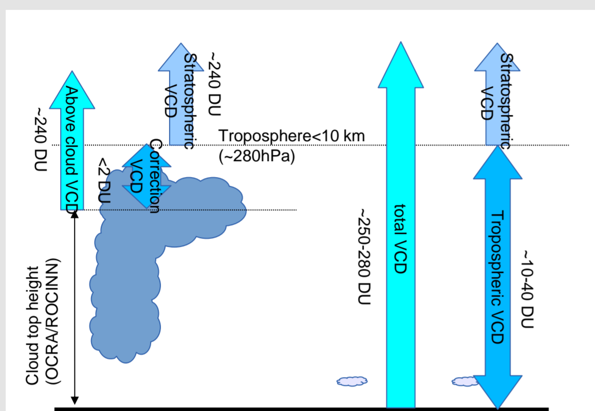
Fig 1: Principle of the convective cloud differential method to retrieve tropospheric ozone column.
