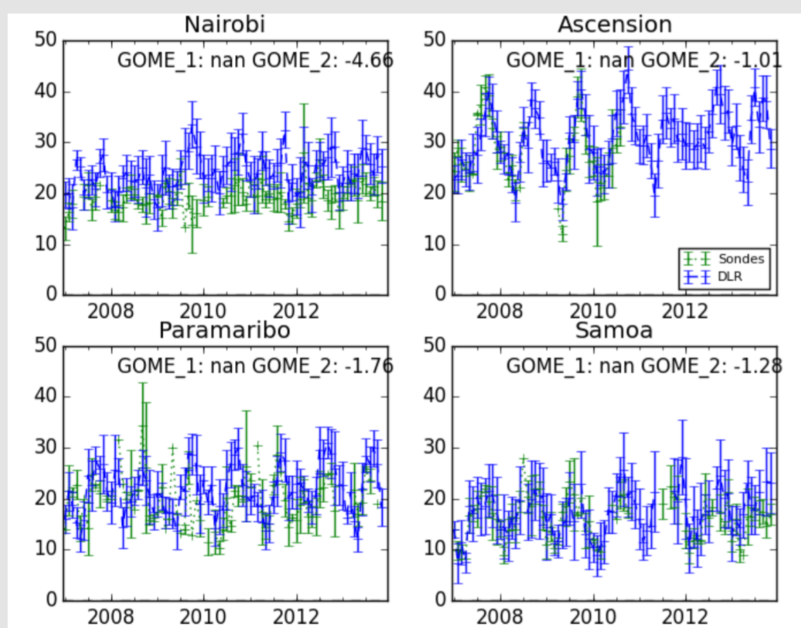
Fig 2: Time series for tropospheric ozone, observed by sondes (green) and GOME_2 on Metop A (blue) for four representative stations.
