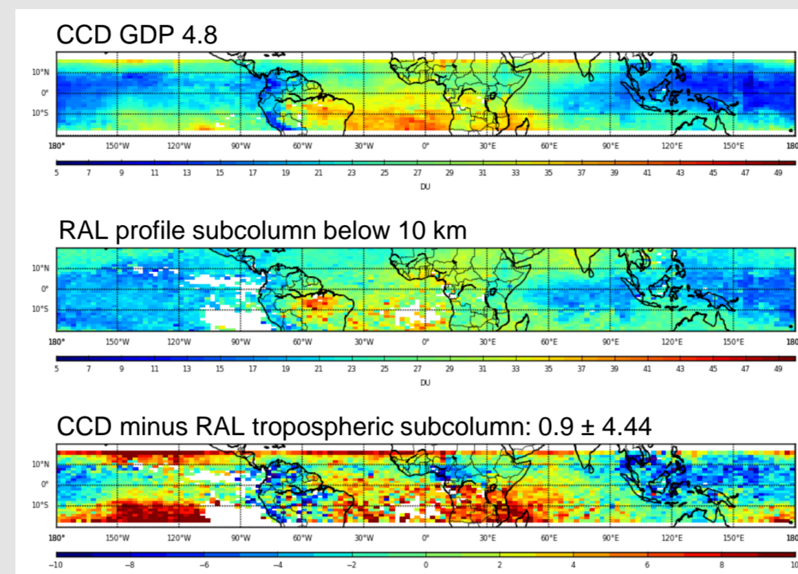
Fig 3: Comparison of GOME_2 CCD data with tropospheric columns below 10 km based on the RAL profile retrieval. Data for Nov 2007
