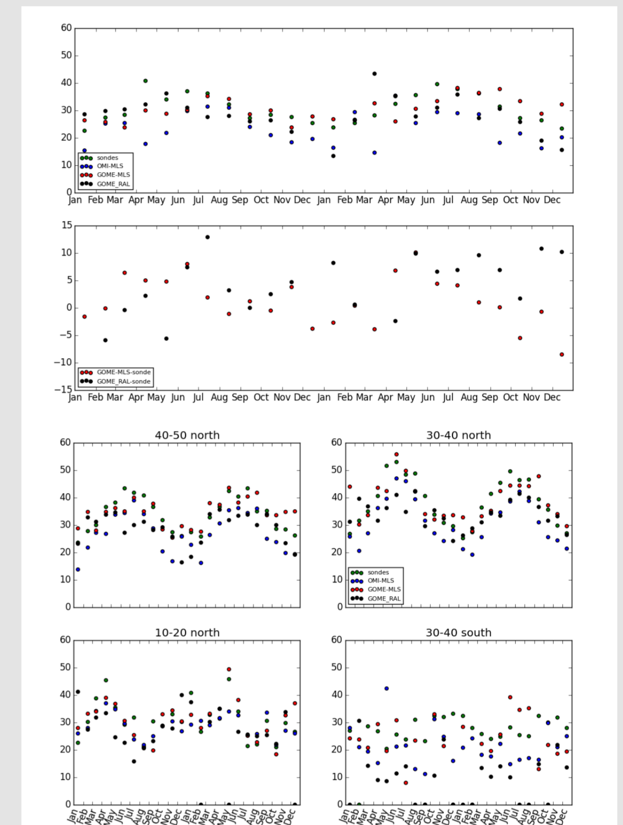
Fig 5 top: Comparison of different ozone column products in DU with the integrated ozone sondes at Hohenpeißenberg for 2007 and 2008.
