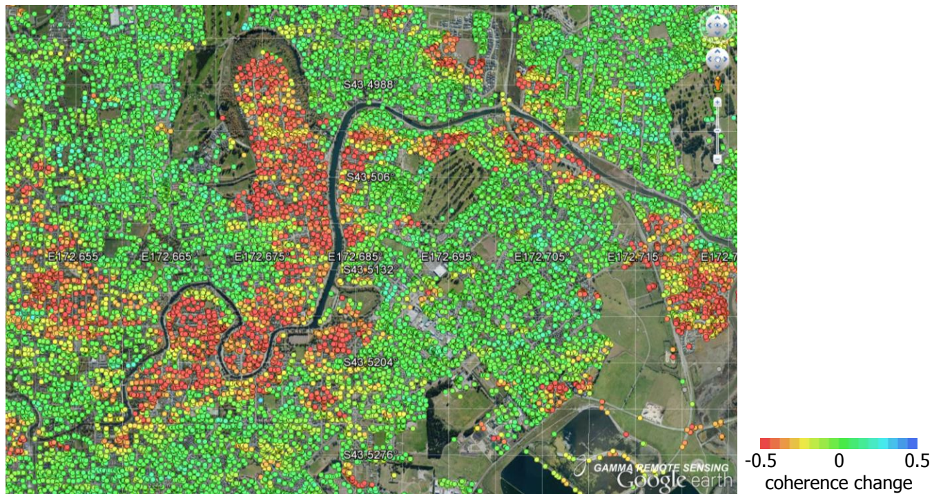
Figure 1. PSI coherence change (red indicates a strong coherence reduction) caused by the Darfield Earthquake on 3-Sep-2010 shown for a section of Christchurch, New Zealand, shown in Google Earth.
