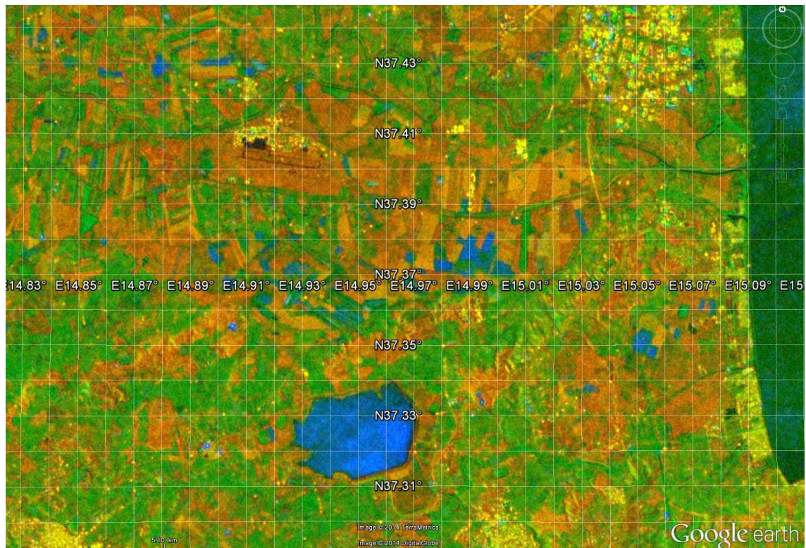
Figure 1 Small section of a Sentinel-1A VV-pol. coherence product derived from IWS data acquired over Sicily on 9. And 21. Aug. 2014. The coherence product is an RGB composite of the interferometric coherence (red), the average backscatter (green) and the backscatter change (blue).
