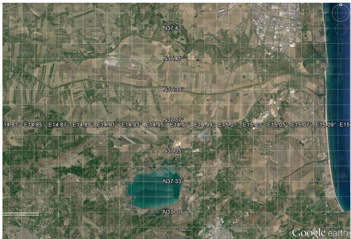
Figure 2 Optical imagery acquired on 29-July-2013 over the area of Figure 1, as found in Google Earth.
